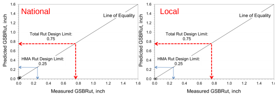
Figure 8. Overall summary of comparisons between measured and predicted granular base layer rutting for HMA pavements
