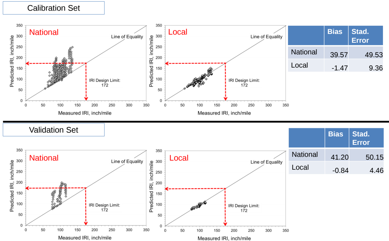
Figure 6. Overall summary of comparisons between measured and predicted JPCP IRI
