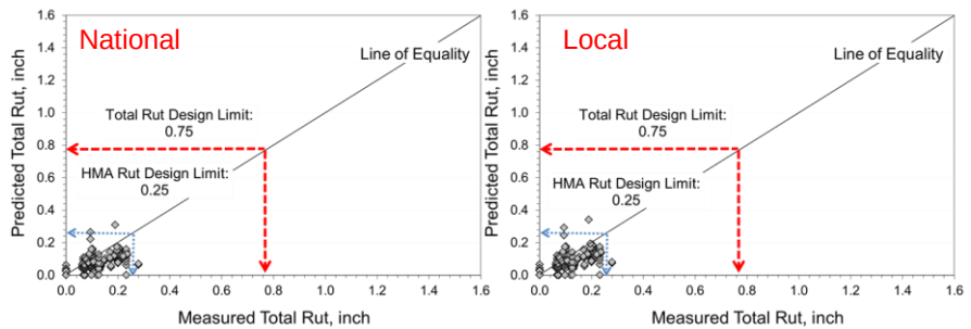
Figure 15. Overall summary of comparisons between measured and predicted total rutting for HMA over JPCP
