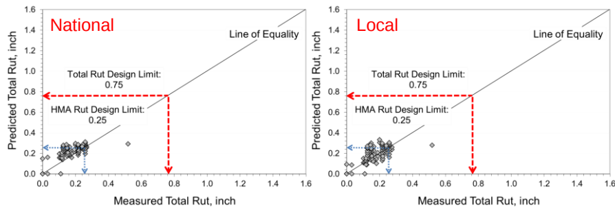
Figure 10. Overall summary of comparisons between measured and predicted total rutting for HMA pavements
