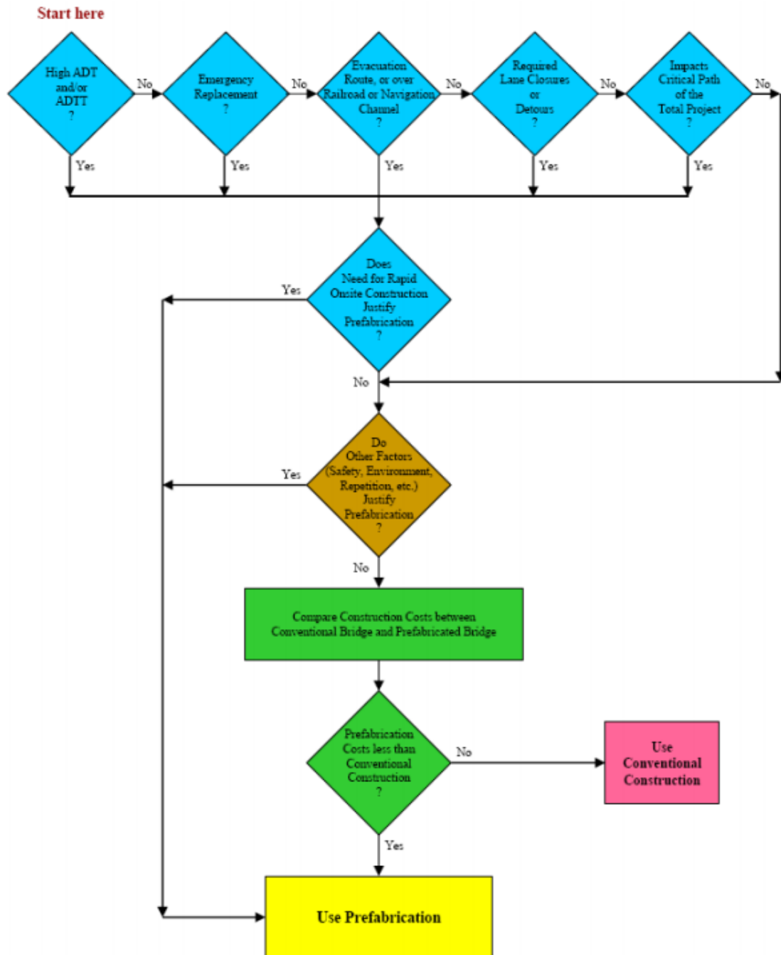
Figure 1. Example of FHWA decision matrix
